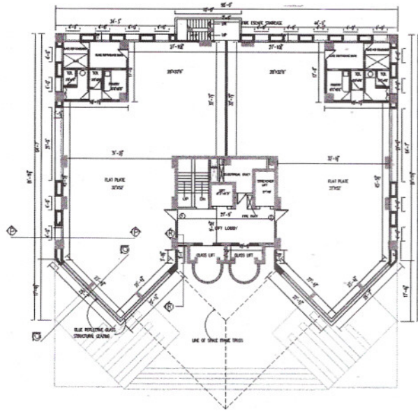
TYPICAL PLAN FOR 5TH TO 9TH FLOOR
